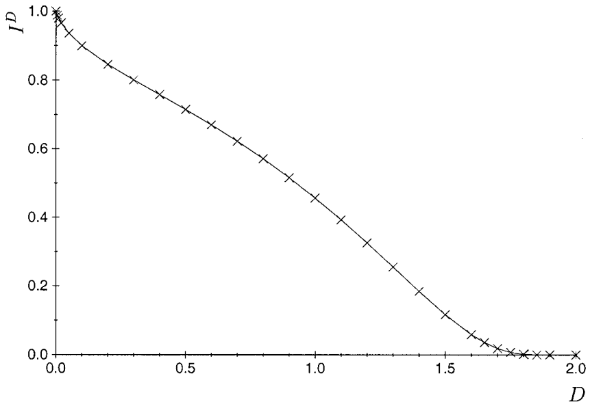
Fig. 4.1. I^D as defined in Eq. (4.40). The crosses have been obtained numerically, the solid line interpolates between these values.
