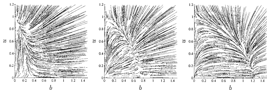
Fig. 4.2. Flow of Eqs. (4.78) for \delta=1 , and \gamma=0.6 , \gamma=1.5 , \gamma=2.5 respectively.
