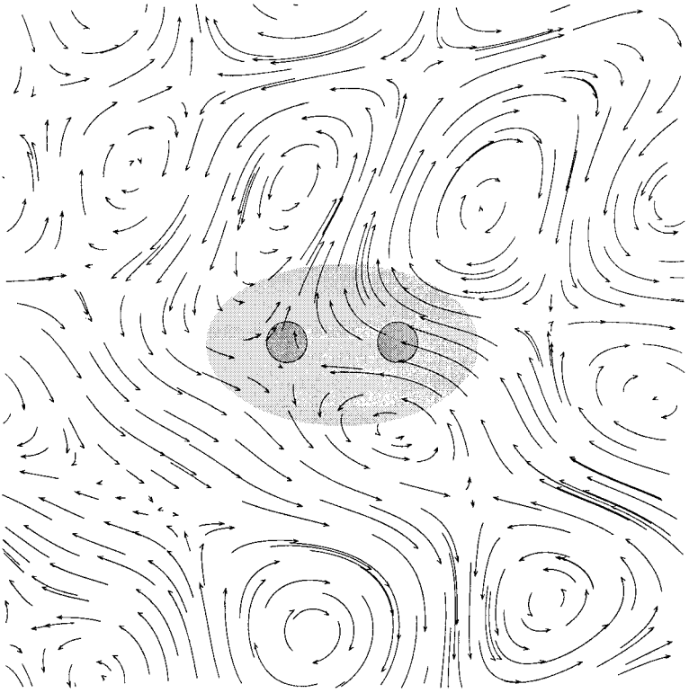
Fig. 1.1. Symbolic picture of a turbulent flow. Particles, or equivalently heat is injected in a finite range of size L \sim 1/M (dark grey areas), whereas the turbulent flow grows up to scale l \sim 1/m , which finally shall be taken to infinity. This is possible, if the total number of particles, or the total heat, injected into the system is conserved. In that case, L and not l sets the largest scale in the problem, and multi-point correlation functions with an anomalous L -dependence will be observable in a domain of size L , here symbolically shaded in light grey. As will be shown below, they have anomalous corrections depending on L .
