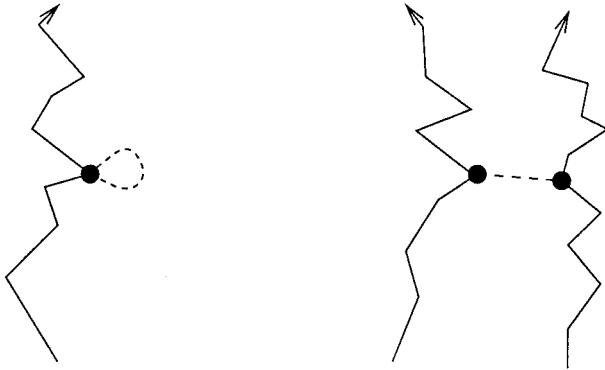
Fig. 3.1. The two different types of diagrams, involved in the renormalization of (a) v (left) and (b) S^{2n} (right). In both cases we have drawn the particle trajectories, as well as one interaction.
