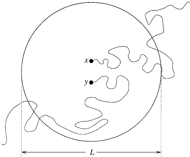
Fig. 3.2. Intuitive interpretation of S^{2n}(x-y) via particles being advected by the turbulent flow. Drown is one configuration which contributed to t_{xy} of Eq. (3.28). Note that particles may return into the box, such that one has to wait long enough until the probability of return tends to 0. For details cmp. the main text.
